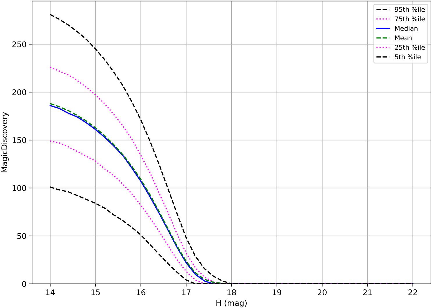
too_elab_heavy_r32_d2_gz_v3.4_10yrs: Trojan 6 detections in 60 nights detection loss
