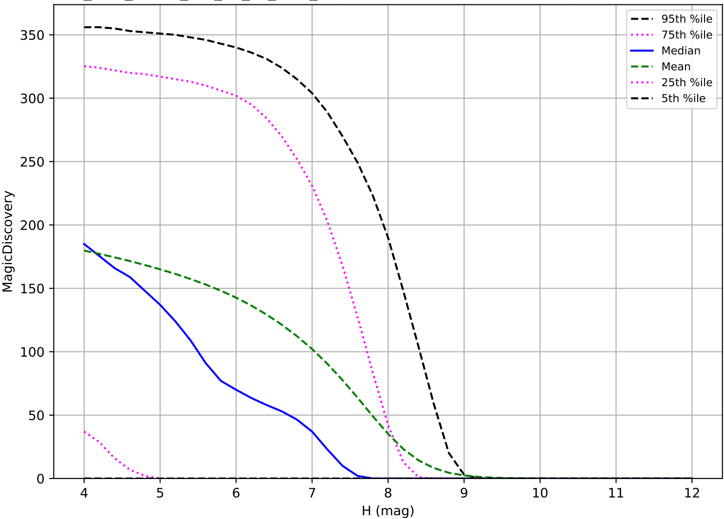
too_elab_heavy_r32_d2_gz_v3.4_10yrs: TNO 6 detections in 60 nights detection loss
