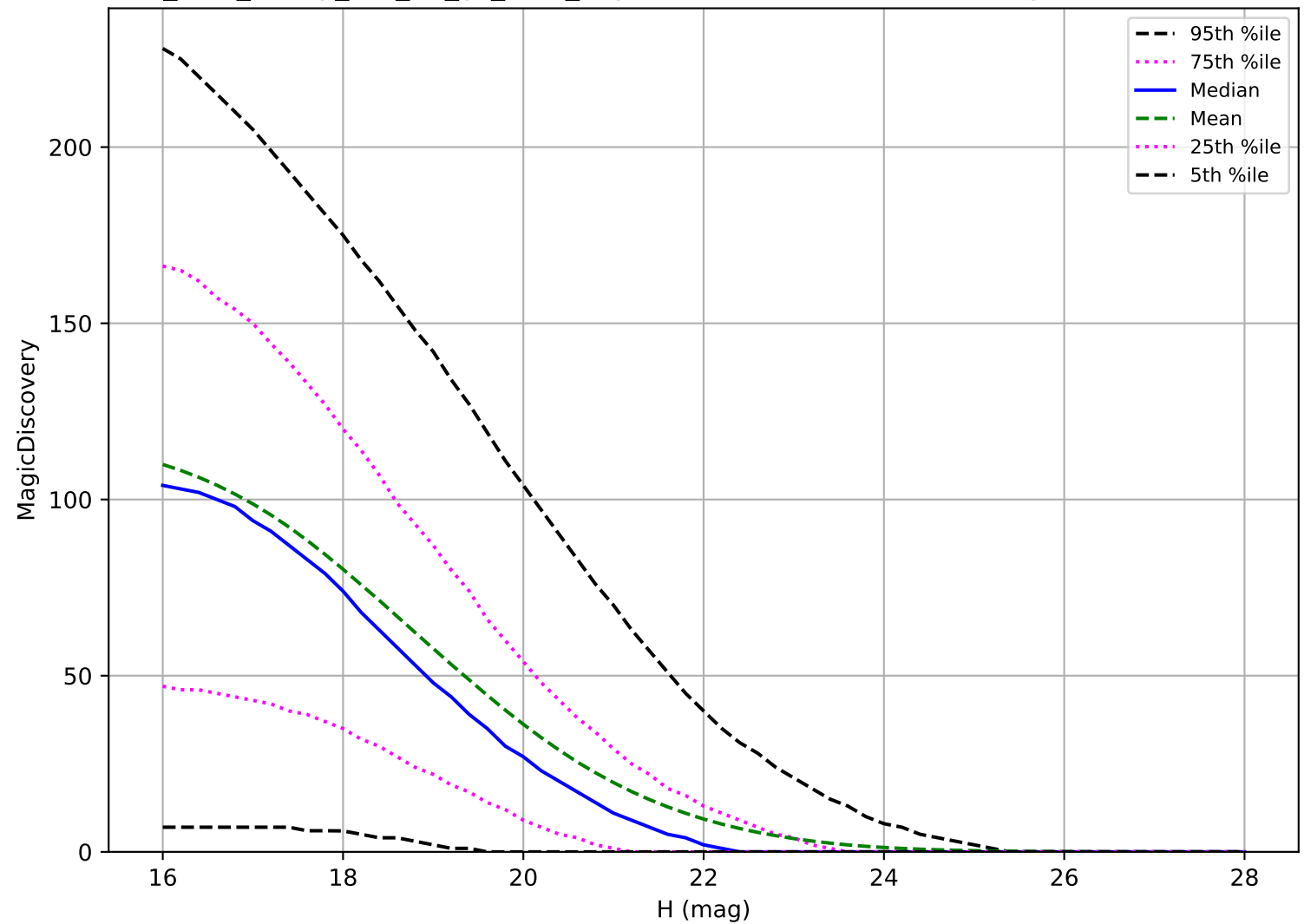
too_elab_heavy_r32_d2_gz_v3.4_10yrs: PHA 6 detections in 60 nights detection loss
