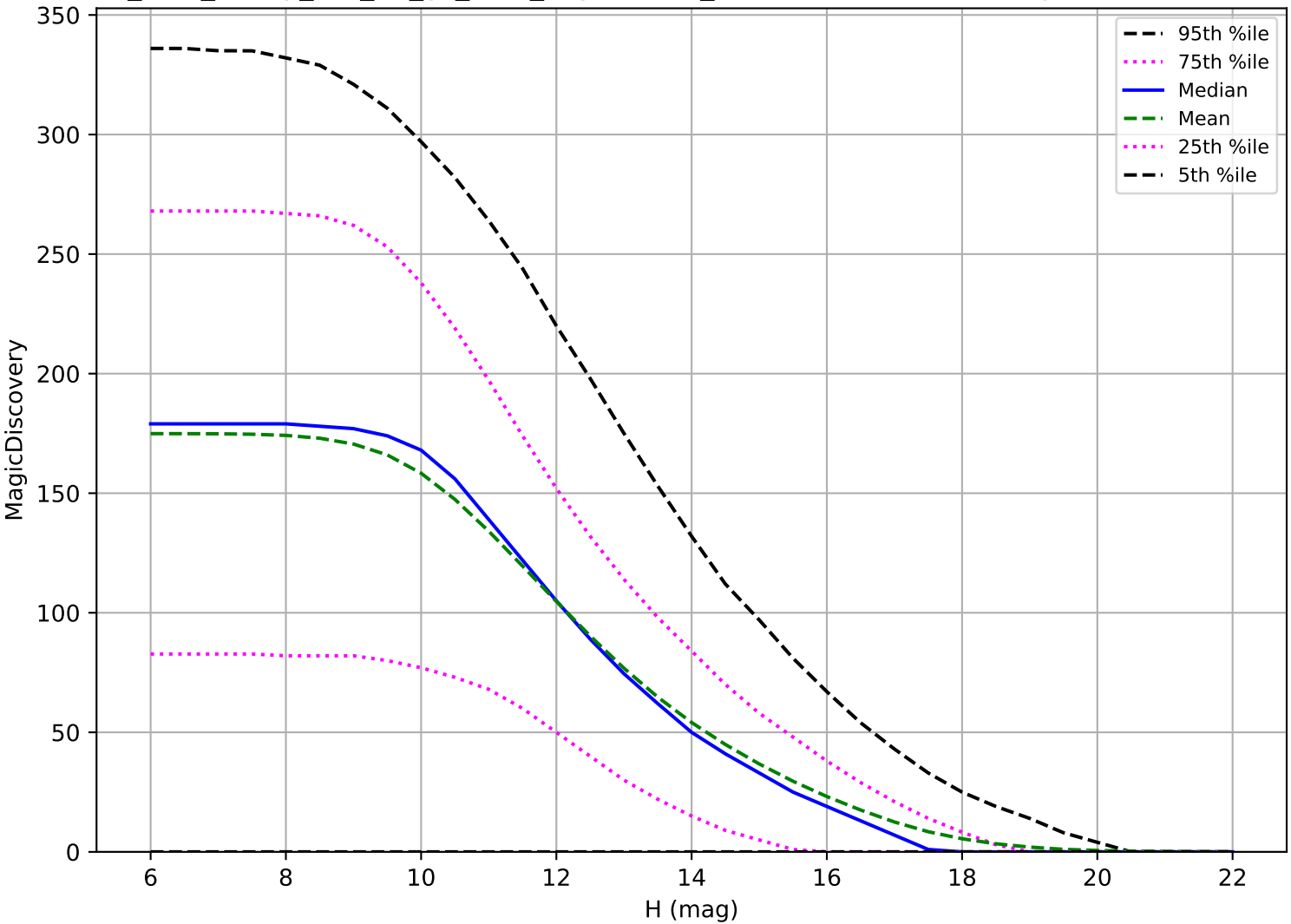
too_elab_heavy_r32_d2_gz_v3.4_10yrs: OCC_r5 6 detections in 60 nights detection loss
