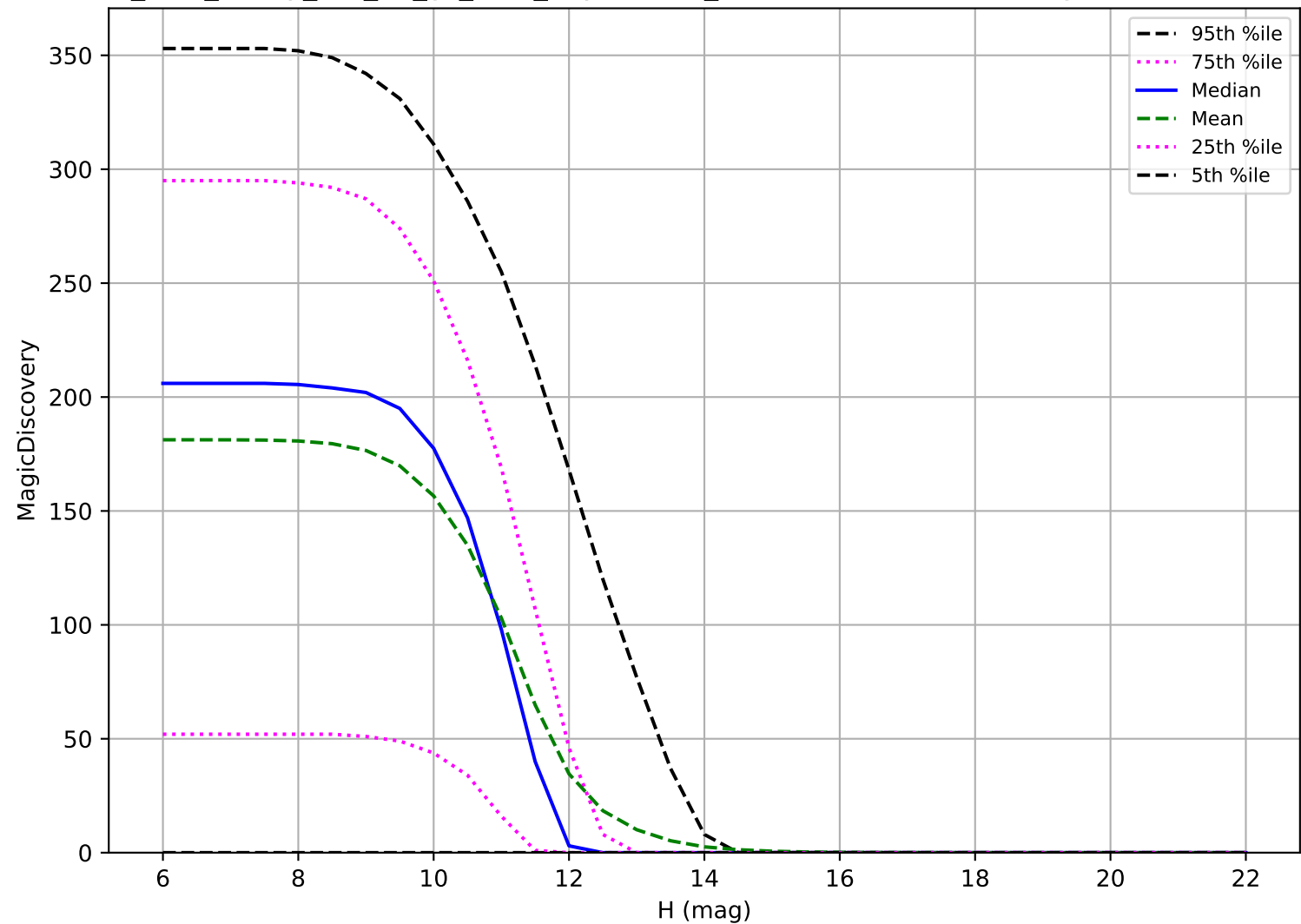
too_elab_heavy_r32_d2_gz_v3.4_10yrs: OCC_r20 6 detections in 60 nights detection loss
