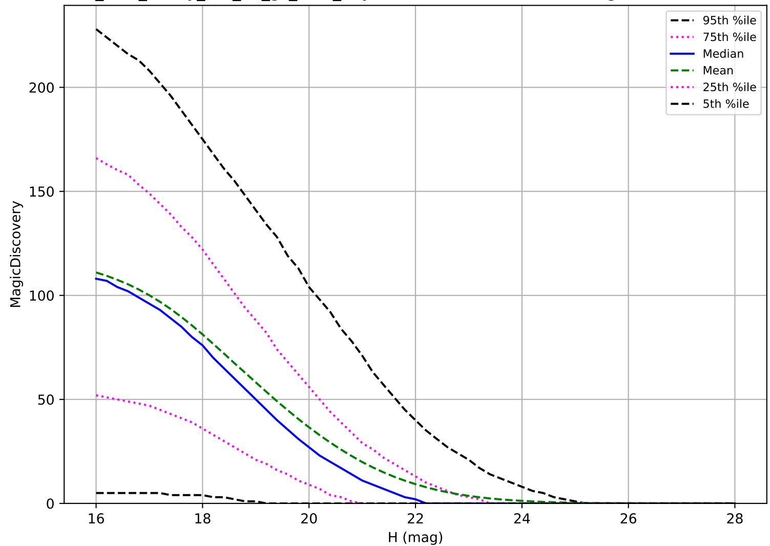
too_elab_heavy_r32_d2_gz_v3.4_10yrs: NEO 6 detections in 60 nights detection loss
