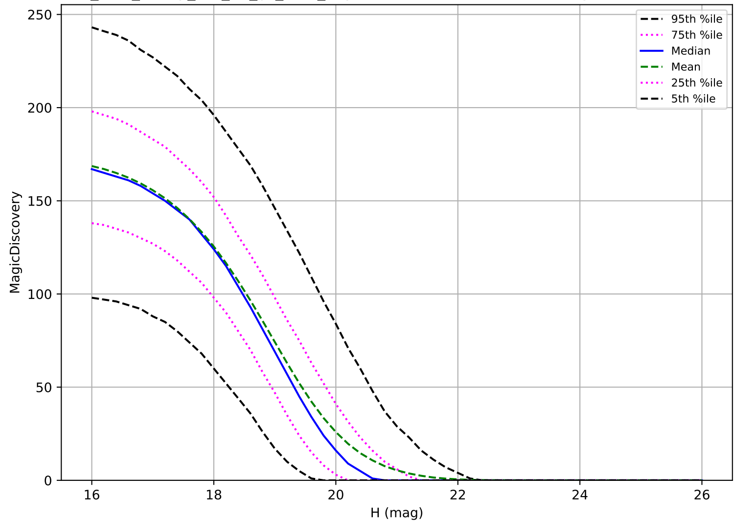
too_elab_heavy_r32_d2_gz_v3.4_10yrs: MBA 6 detections in 60 nights detection loss
