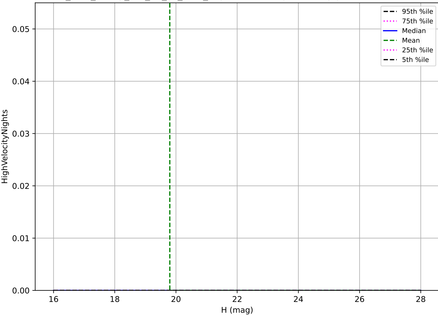
too_elab_heavy_r32_d2_gz_v3.4_10yrs: Vatira High velocity pair detection loss
