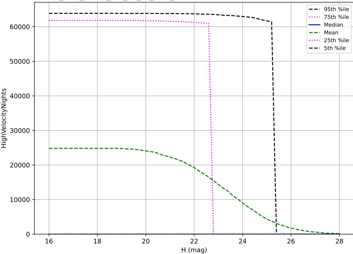
too_elab_heavy_r32_d2_gz_v3.4_10yrs: PHA High velocity pair detection loss
