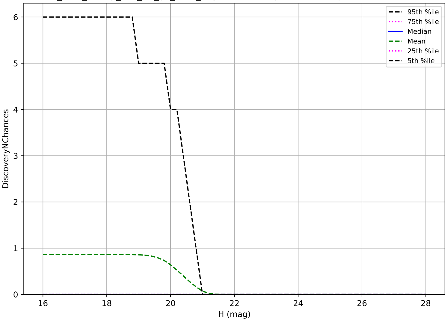
too_elab_heavy_r32_d2_gz_v3.4_10yrs: Vatira 3 pairs in 15 nights detection loss
