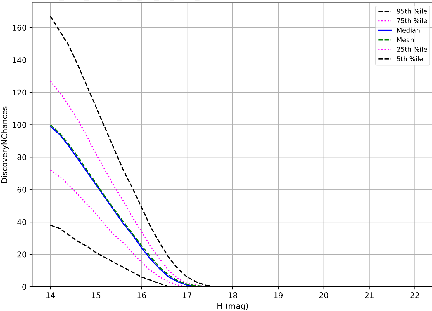
too_elab_heavy_r32_d2_gz_v3.4_10yrs: Trojan 3 pairs in 15 nights detection loss
