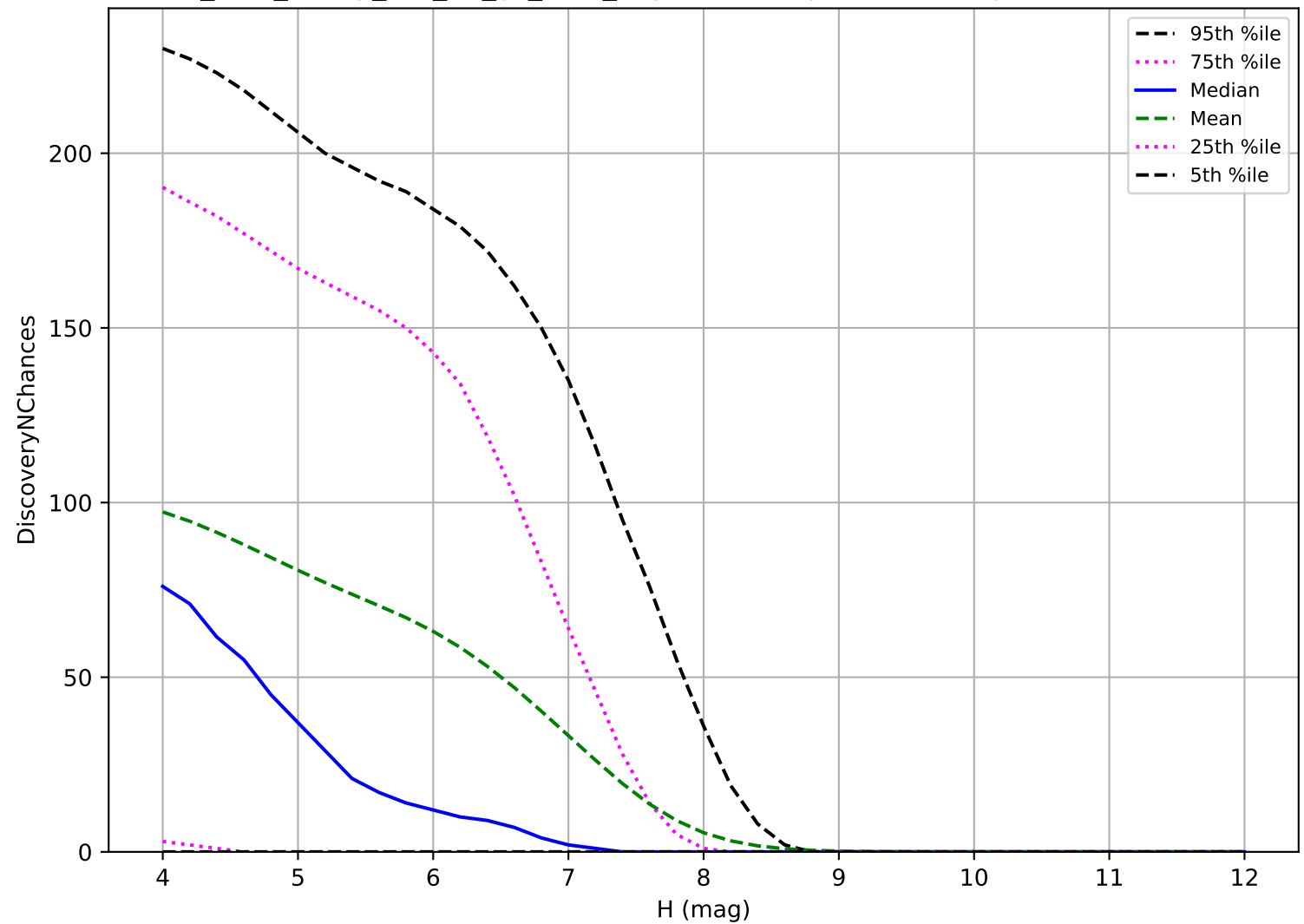
too_elab_heavy_r32_d2_gz_v3.4_10yrs: TNO 3 pairs in 15 nights detection loss
