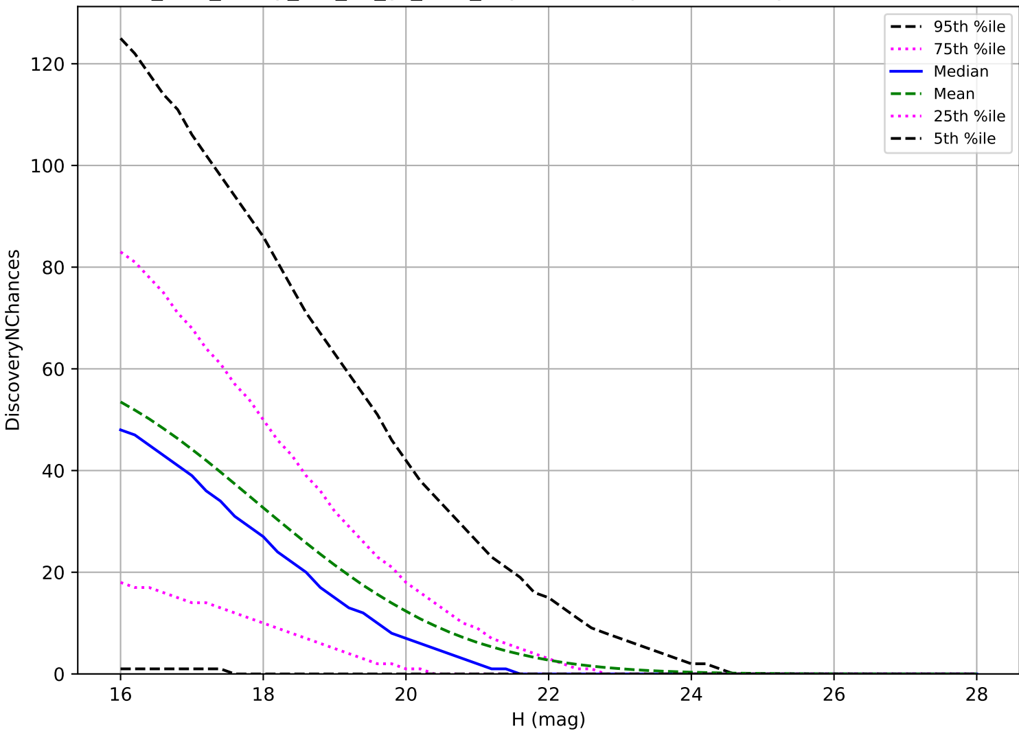
too_elab_heavy_r32_d2_gz_v3.4_10yrs: PHA 3 pairs in 15 nights detection loss
