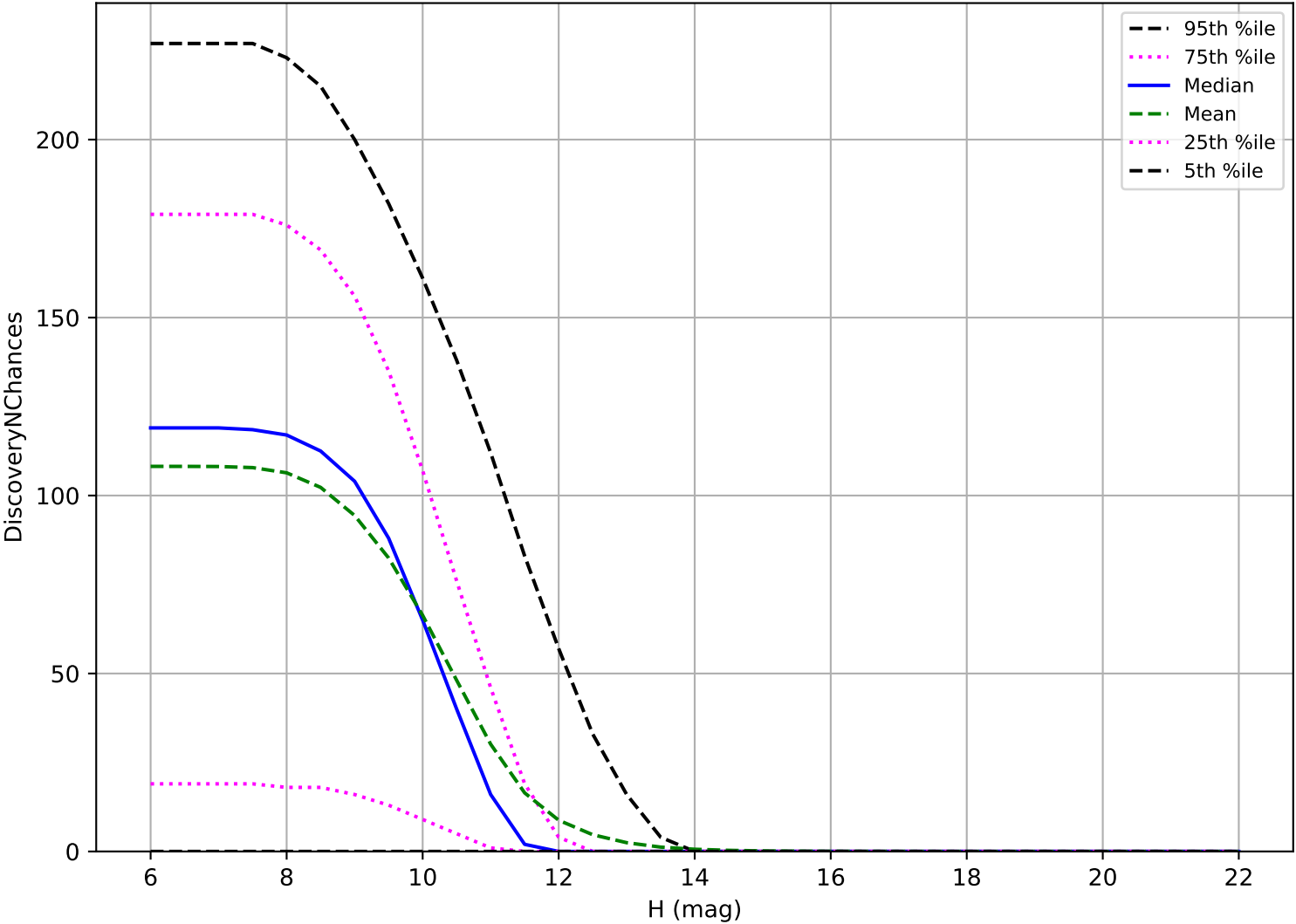
too_elab_heavy_r32_d2_gz_v3.4_10yrs: OCC_r20 3 pairs in 15 nights detection loss
