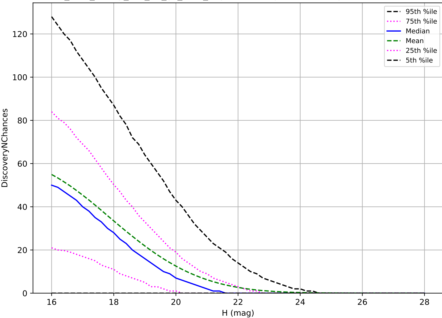
too_elab_heavy_r32_d2_gz_v3.4_10yrs: NEO 3 pairs in 15 nights detection loss
