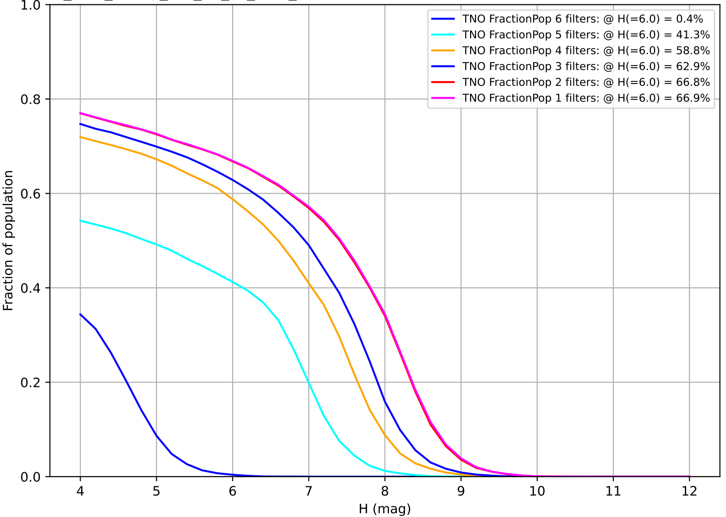
too_elab_heavy_r32_d2_gz_v3.4_10yrs: Fraction of population with colors in X filters TNO
