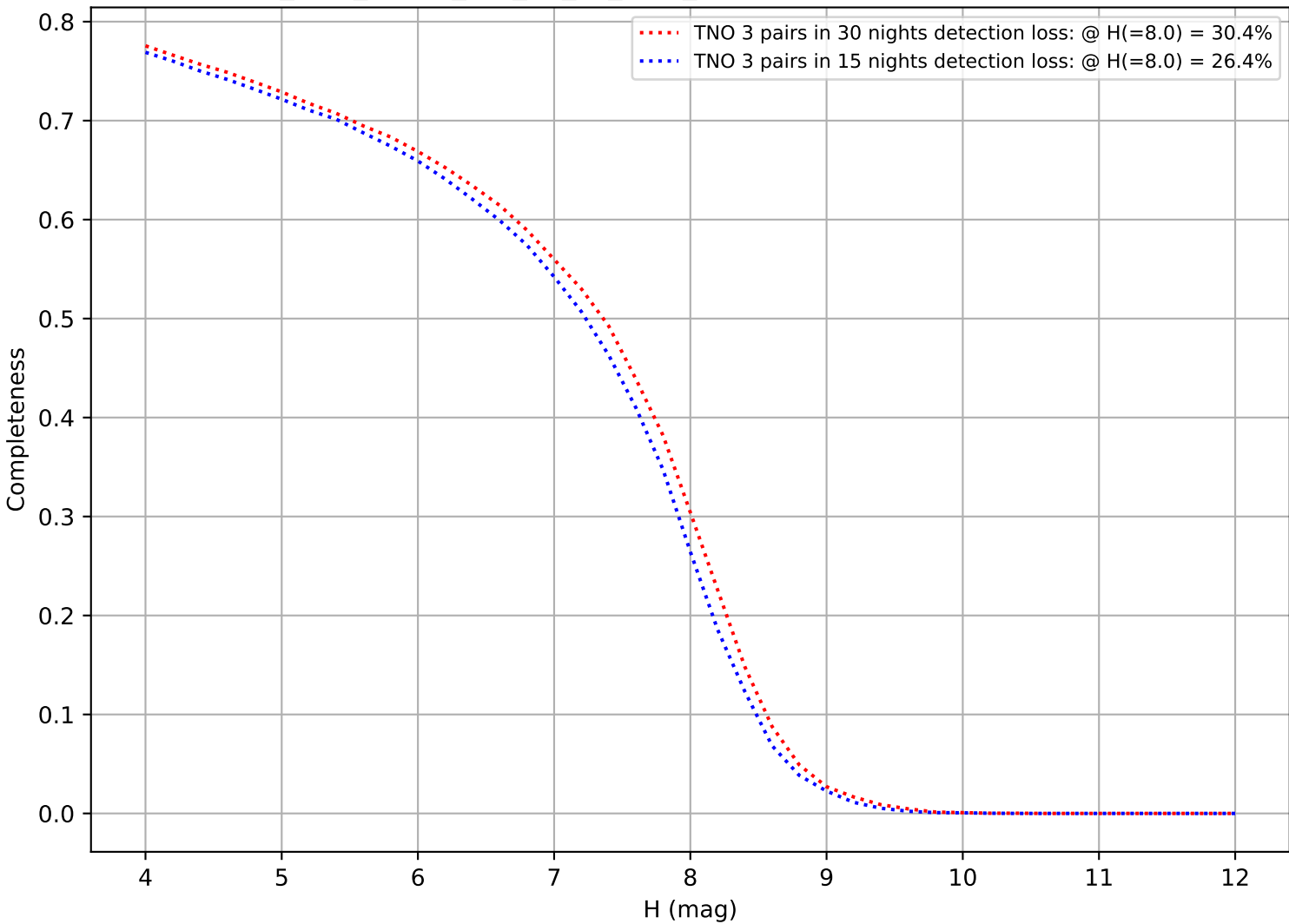
too_elab_heavy_r32_d2_gz_v3.4_10yrs: DifferentialCompleteness
