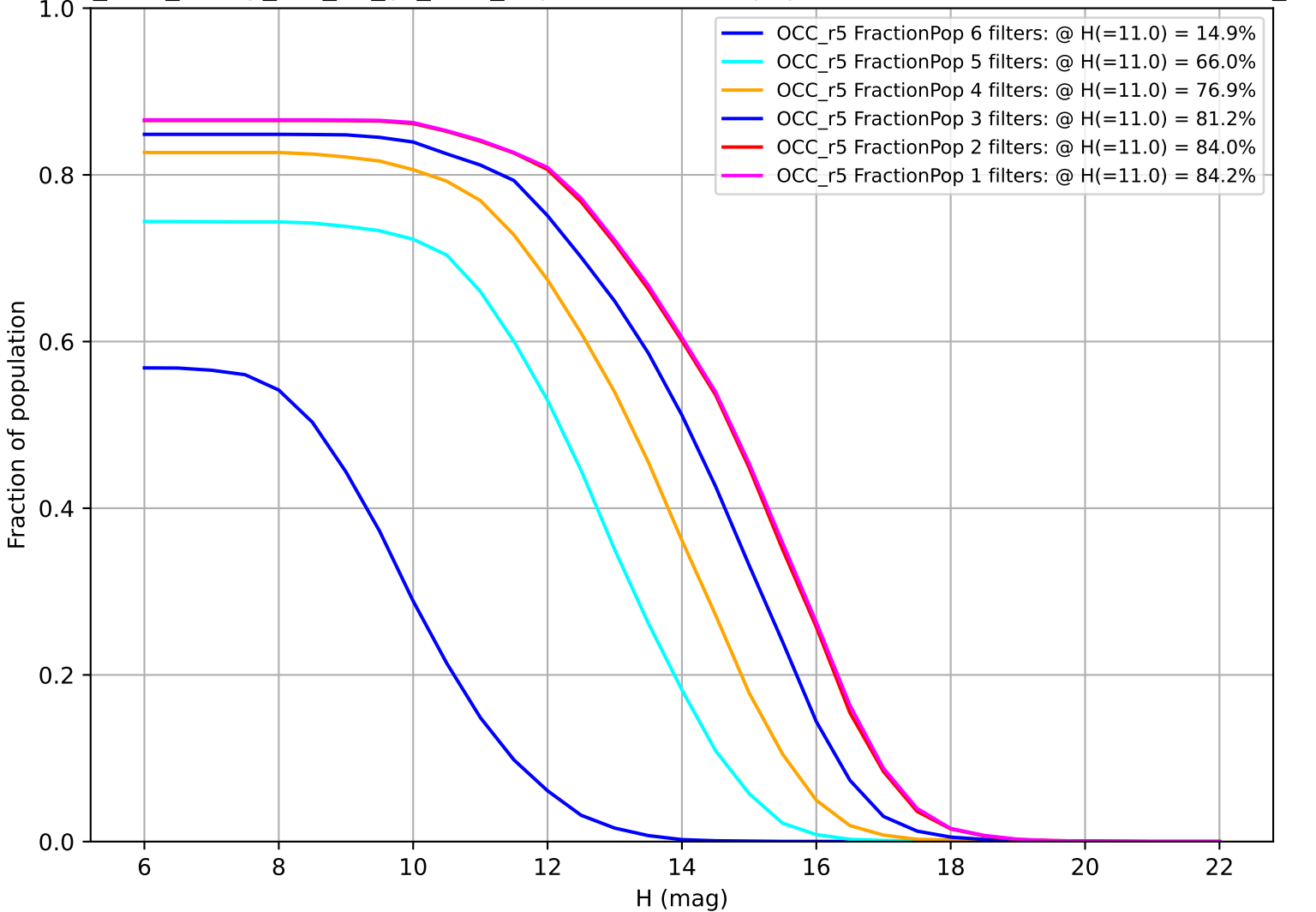
too_elab_heavy_r32_d2_gz_v3.4_10yrs: Fraction of population with colors in X filters OCC_r5
