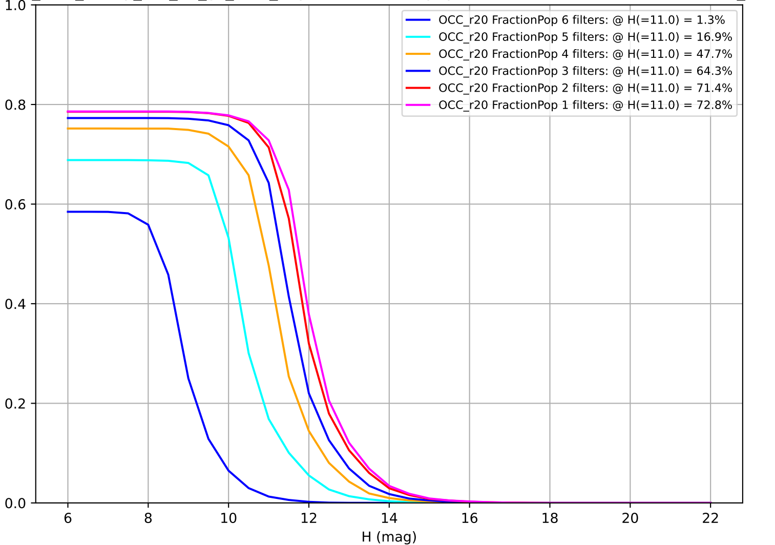
too_elab_heavy_r32_d2_gz_v3.4_10yrs: Fraction of population with colors in X filters OCC_r20
