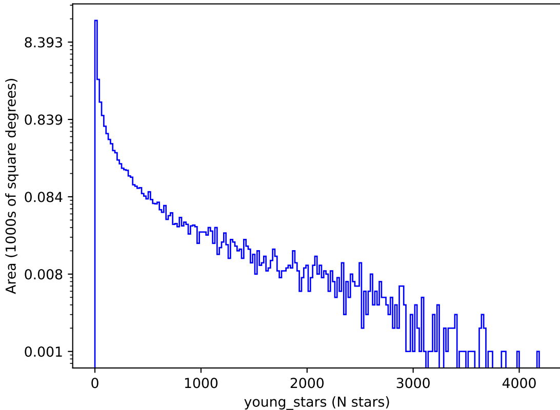
too_elab_heavy_r32_d2_gz_v3.4_10yrs : young_stars
