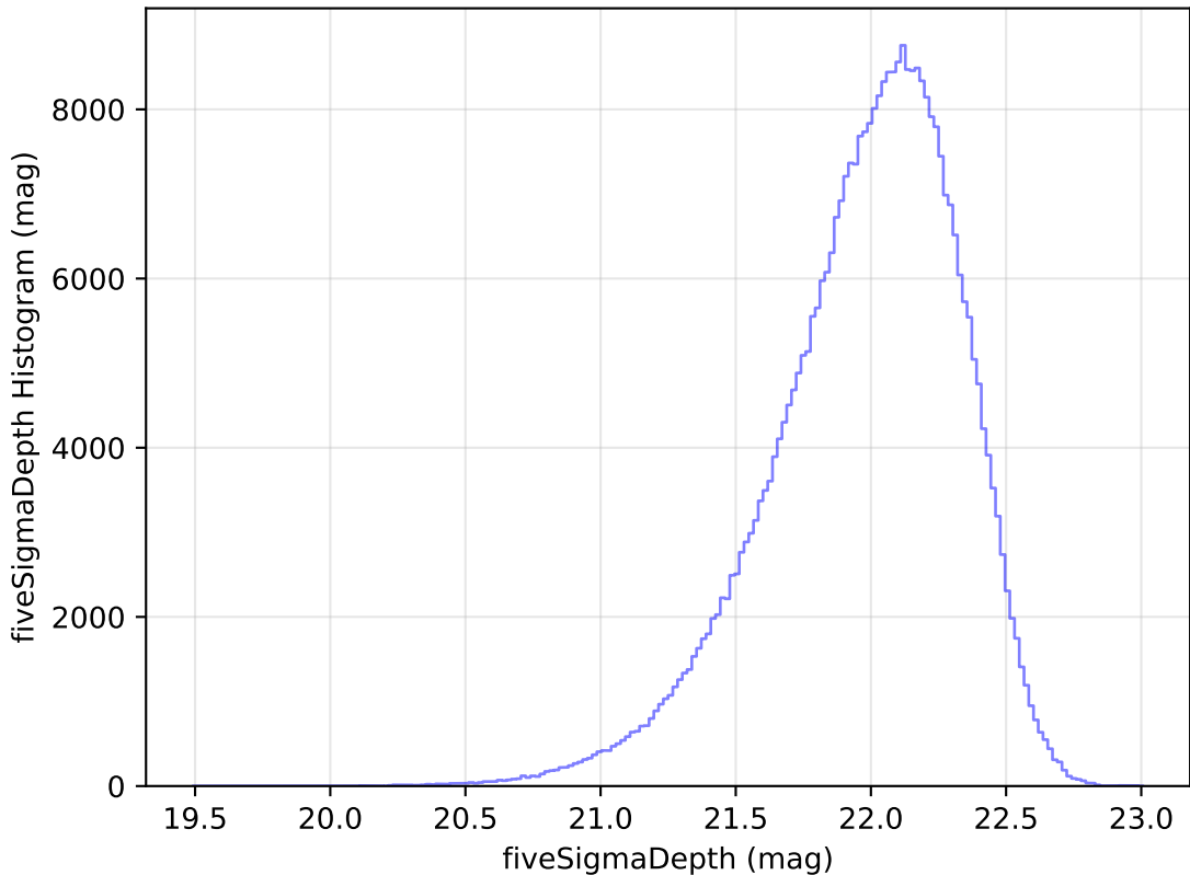
too_elab_heavy_r32_d2_gz_v3.4_10yrs y: fiveSigmaDepth Histogram
