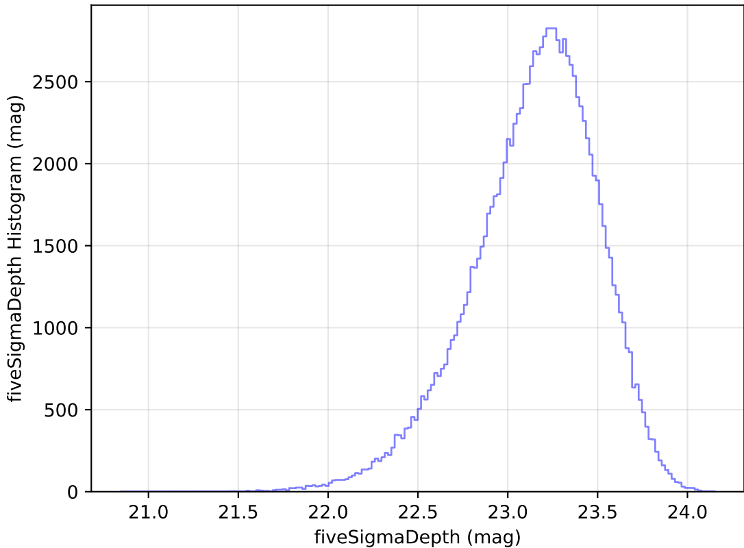
too_elab_heavy_r32_d2_gz_v3.4_10yrs u: fiveSigmaDepth Histogram
