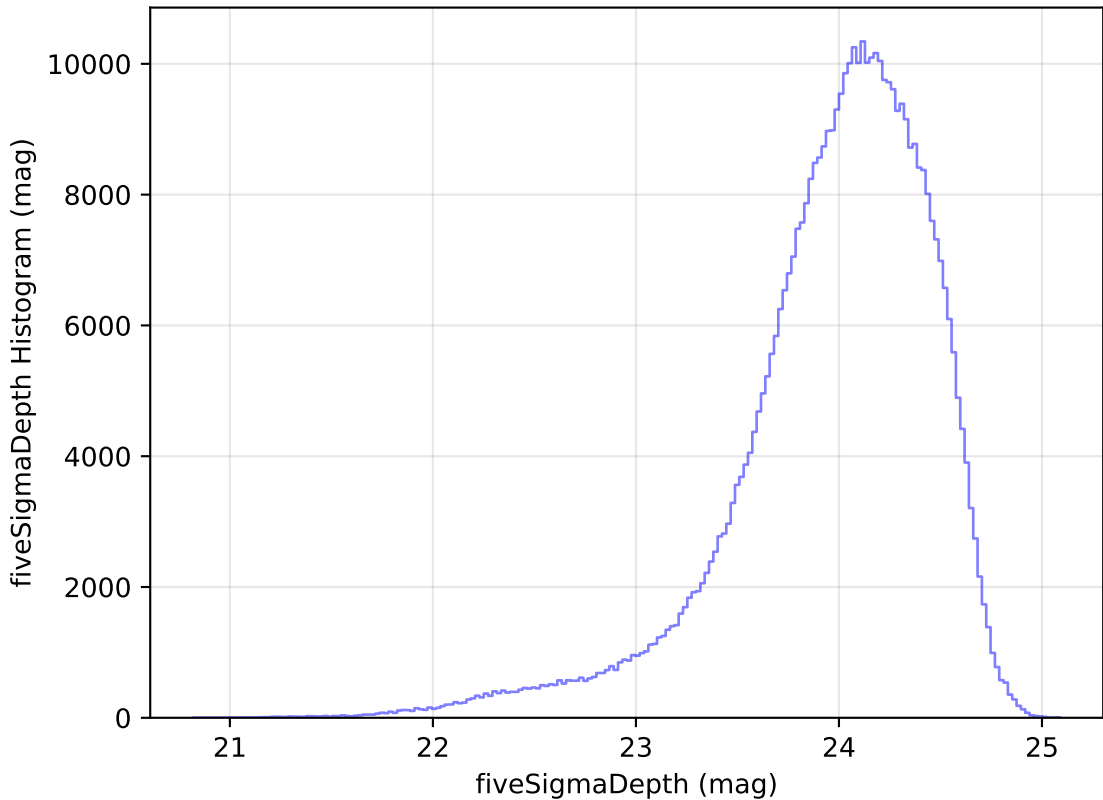
too_elab_heavy_r32_d2_gz_v3.4_10yrs r: fiveSigmaDepth Histogram
