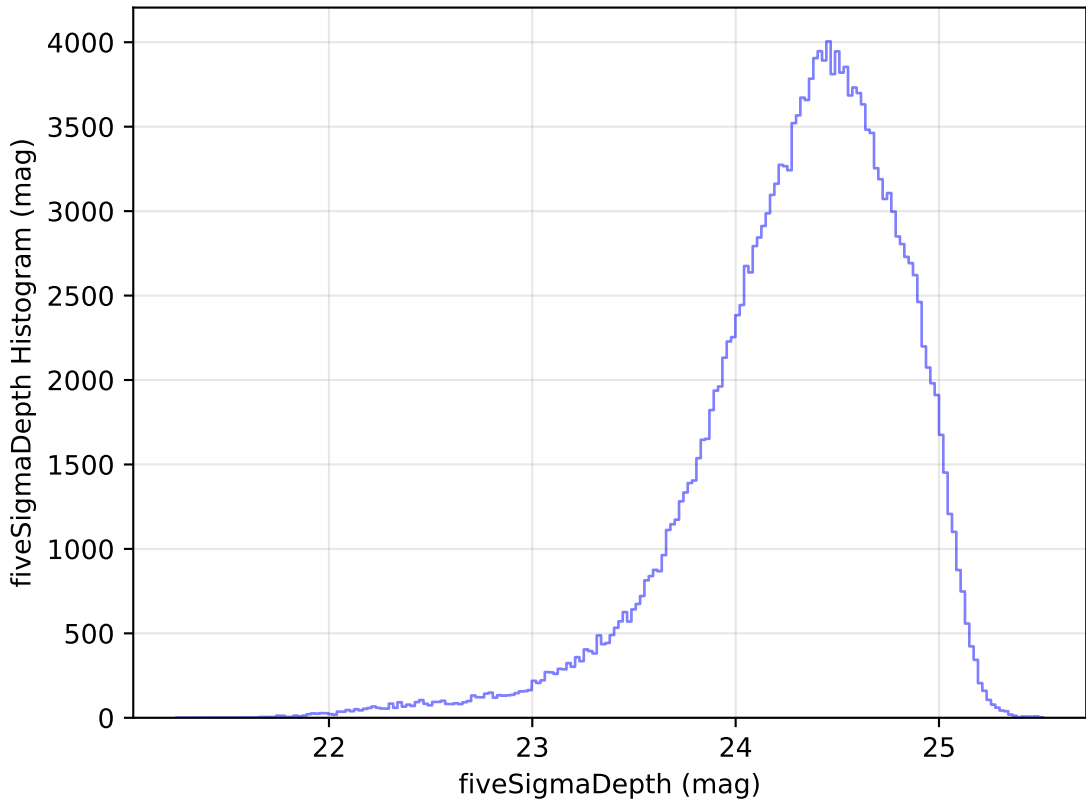
too_elab_heavy_r32_d2_gz_v3.4_10yrs g: fiveSigmaDepth Histogram
