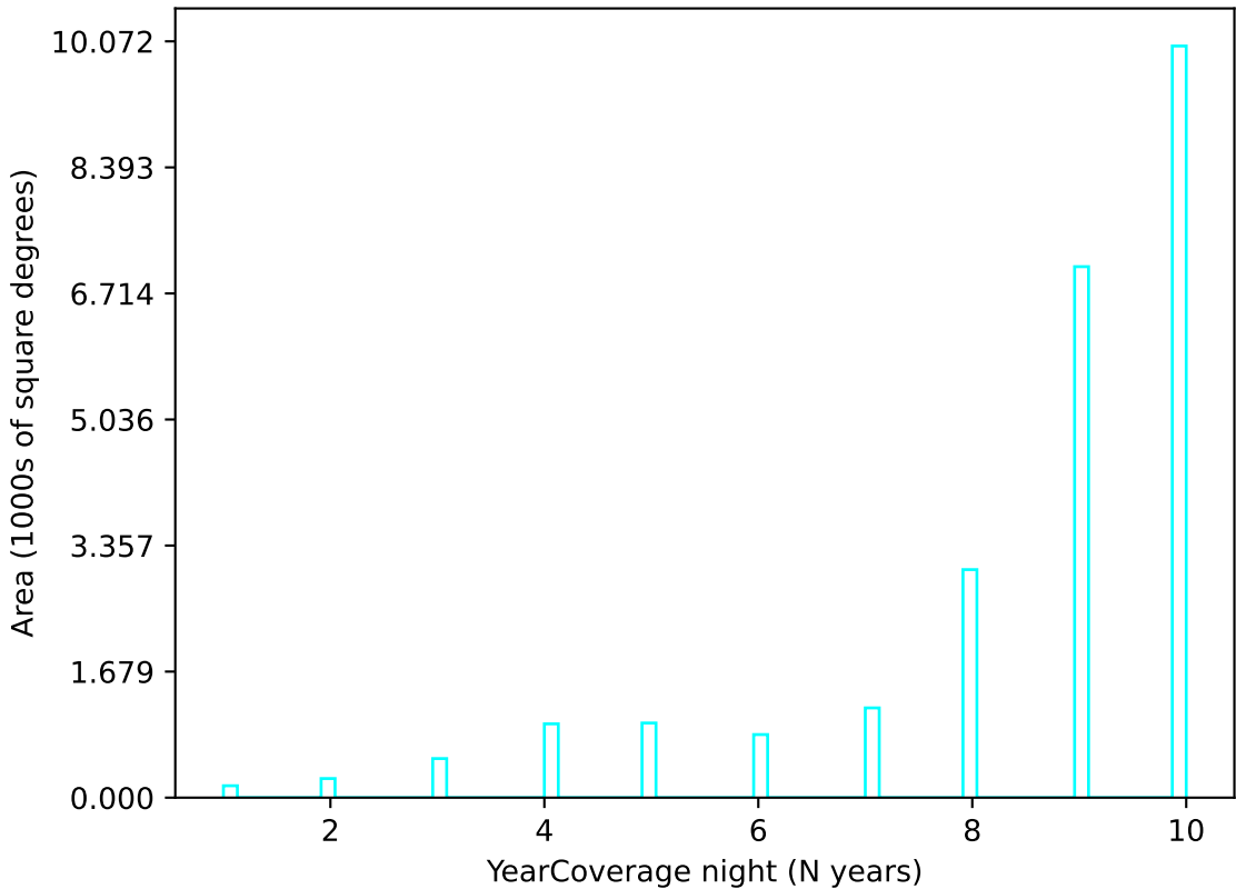
too_elab_heavy_r32_d2_gz_v3.4_10yrs u band: YearCoverage night
