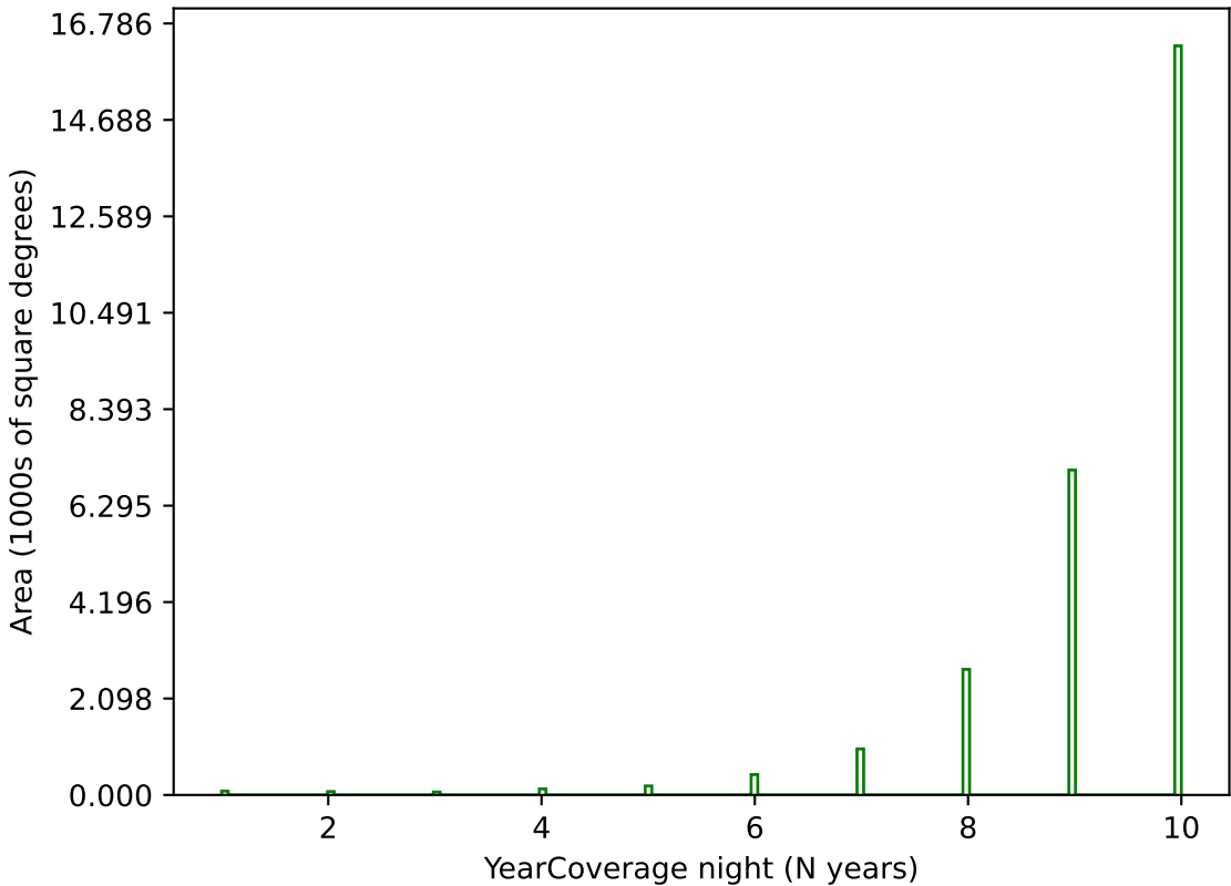
too_elab_heavy_r32_d2_gz_v3.4_10yrs g band: YearCoverage night
