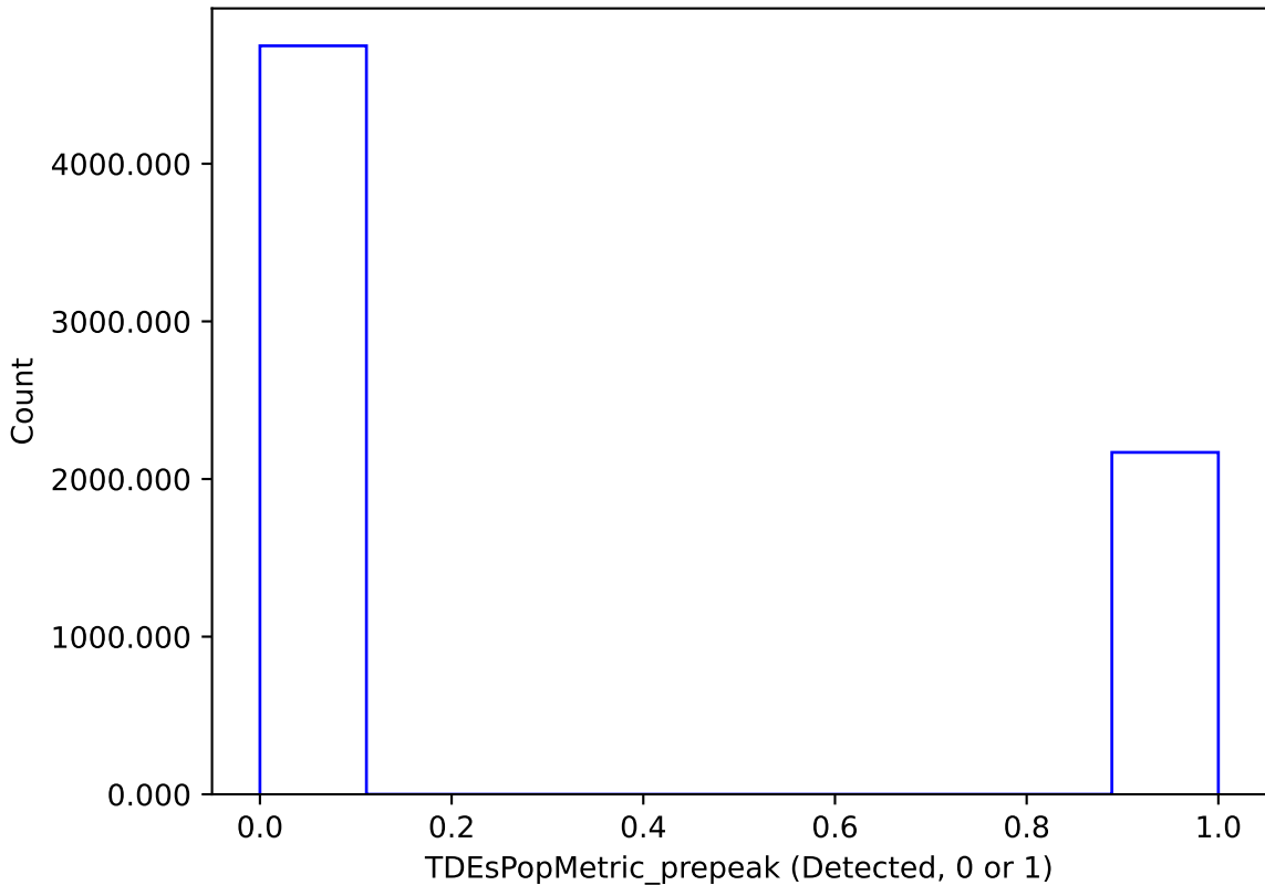
too_elab_heavy_r32_d2_gz_v3.4_10yrs : TDEsPopMetric_prepeak
