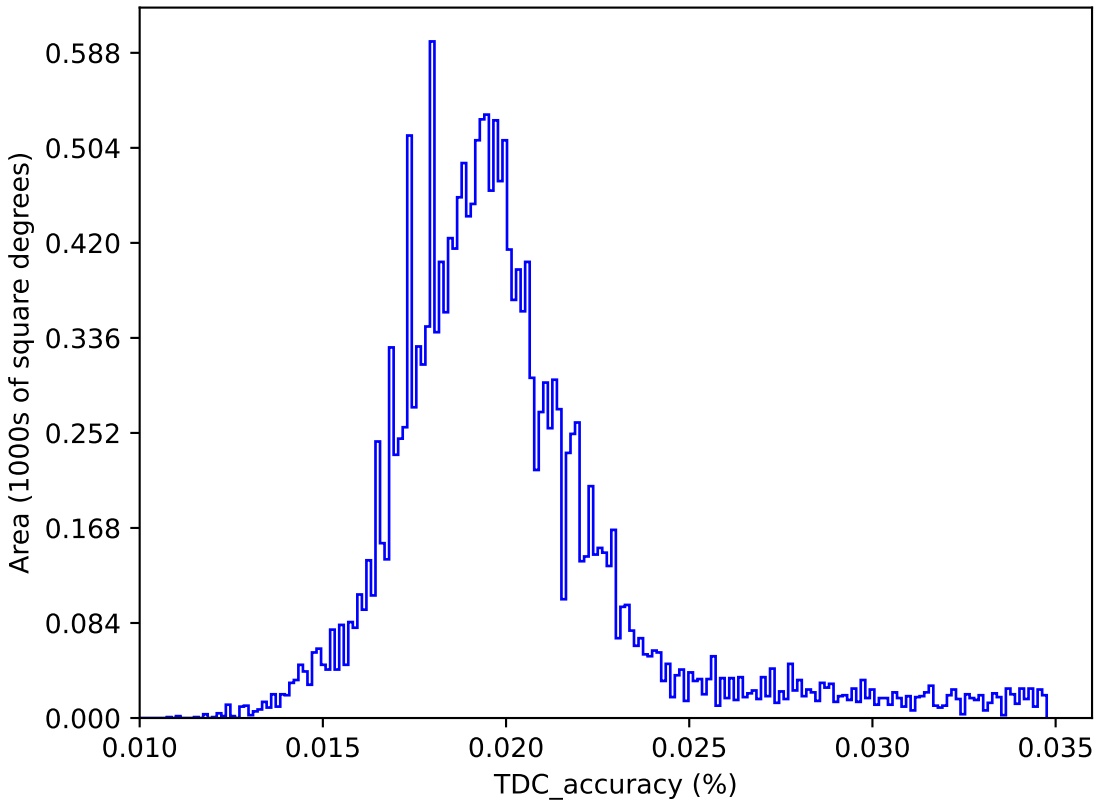
too_elab_heavy_r32_d2_gz_v3.4_10yrs : TDC_accuracy
