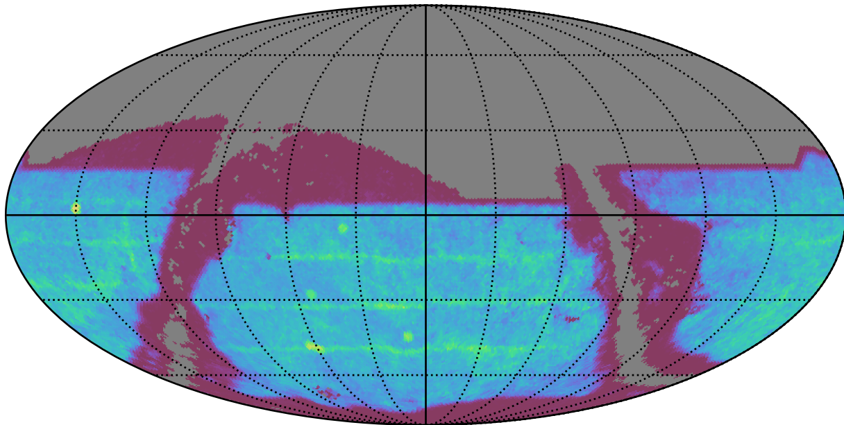
too_elab_heavy_r32_d2_gz_v3.4_10yrs : SNSLMetric
