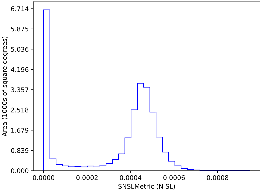
too_elab_heavy_r32_d2_gz_v3.4_10yrs : SNSLMetric
