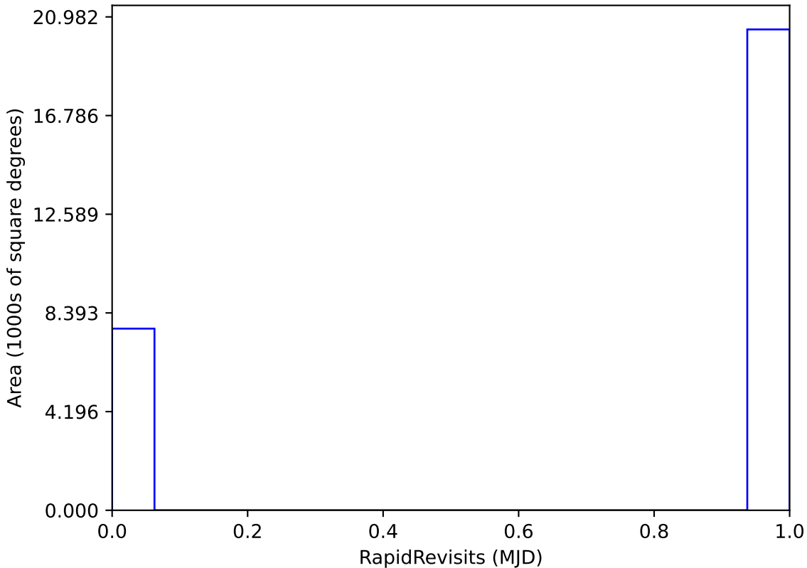
too_elab_heavy_r32_d2_gz_v3.4_10yrs : RapidRevisits
