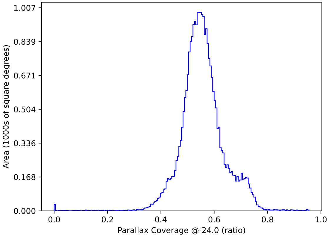
too_elab_heavy_r32_d2_gz_v3.4_10yrs : Parallax Coverage @ 24.0
