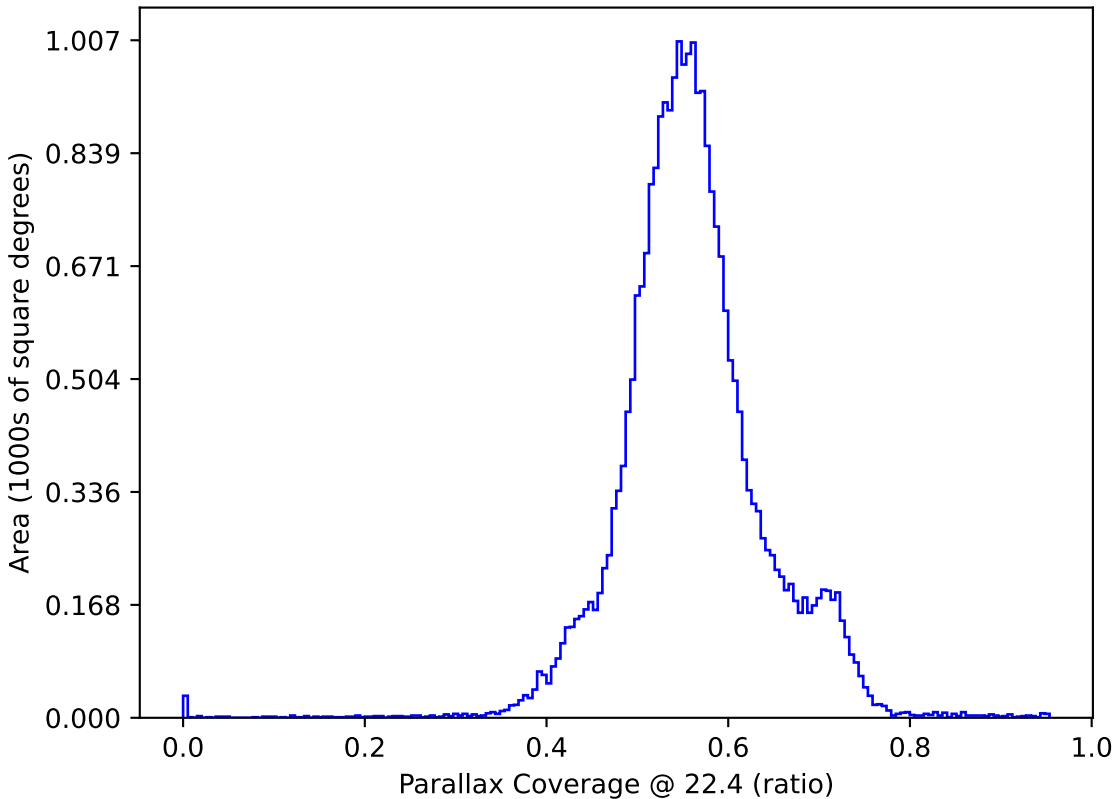
too_elab_heavy_r32_d2_gz_v3.4_10yrs : Parallax Coverage @ 22.4
