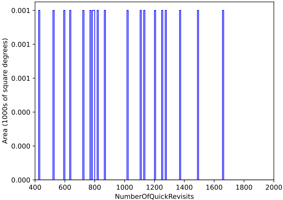
too_elab_heavy_r32_d2_gz_v3.4_10yrs : NumberOfQuickRevisits
