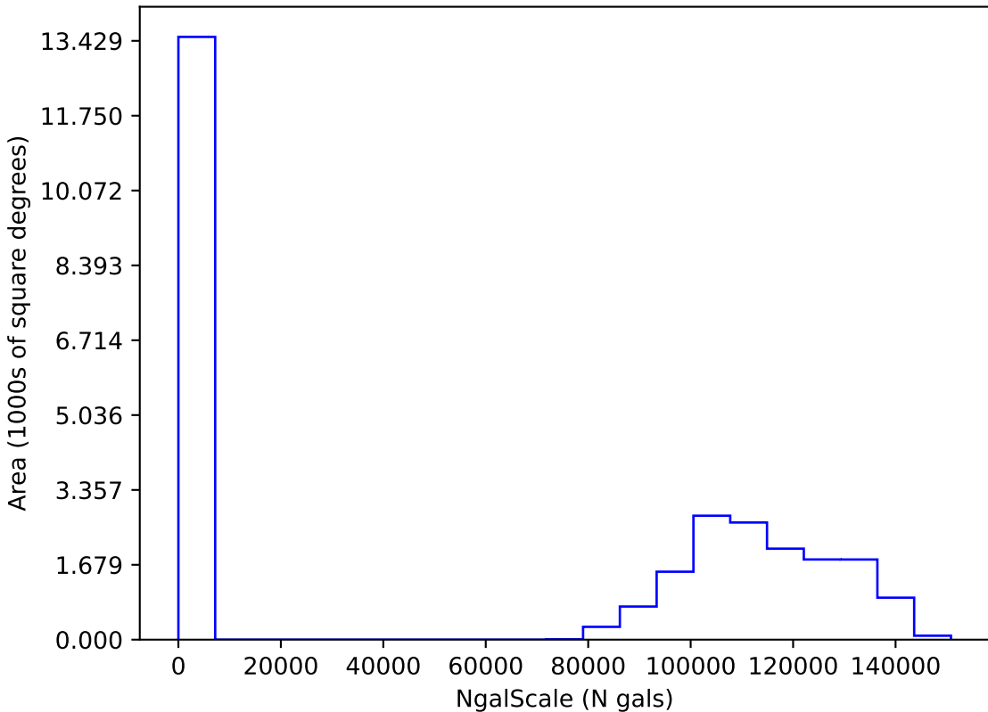
too_elab_heavy_r32_d2_gz_v3.4_10yrs i: NgalScale
