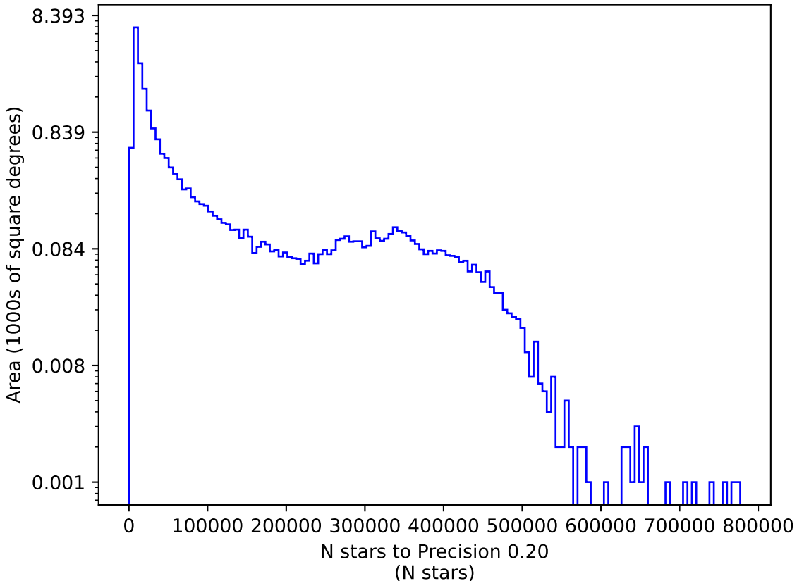
too_elab_heavy_r32_d2_gz_v3.4_10yrs y: N stars to Precision 0.20
