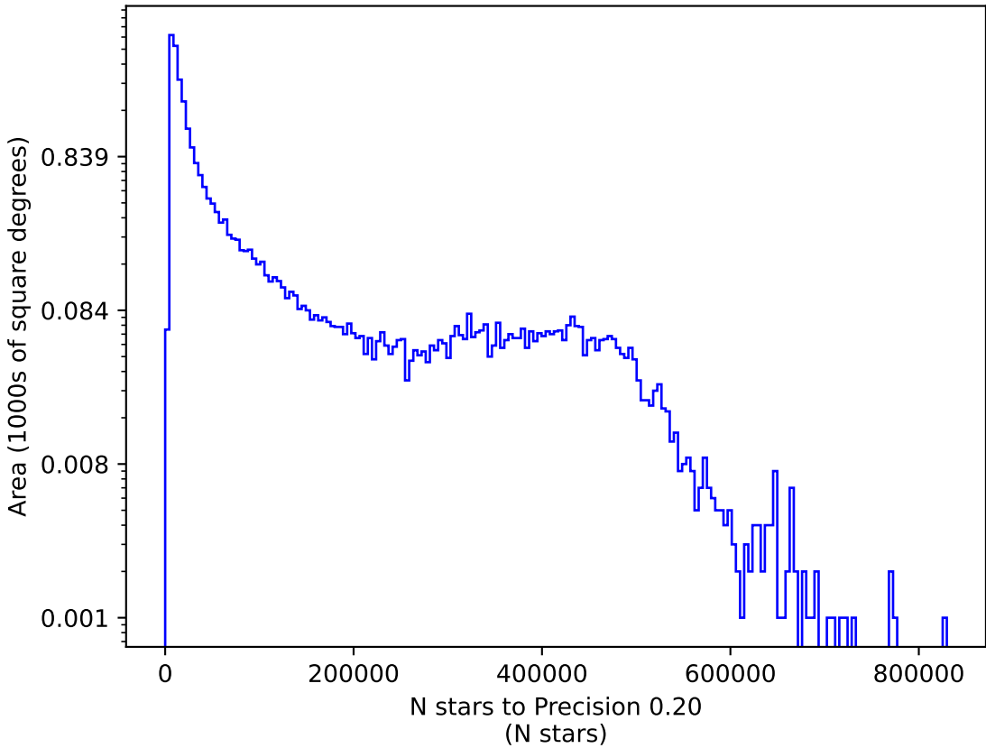
too_elab_heavy_r32_d2_gz_v3.4_10yrs r: N stars to Precision 0.20
