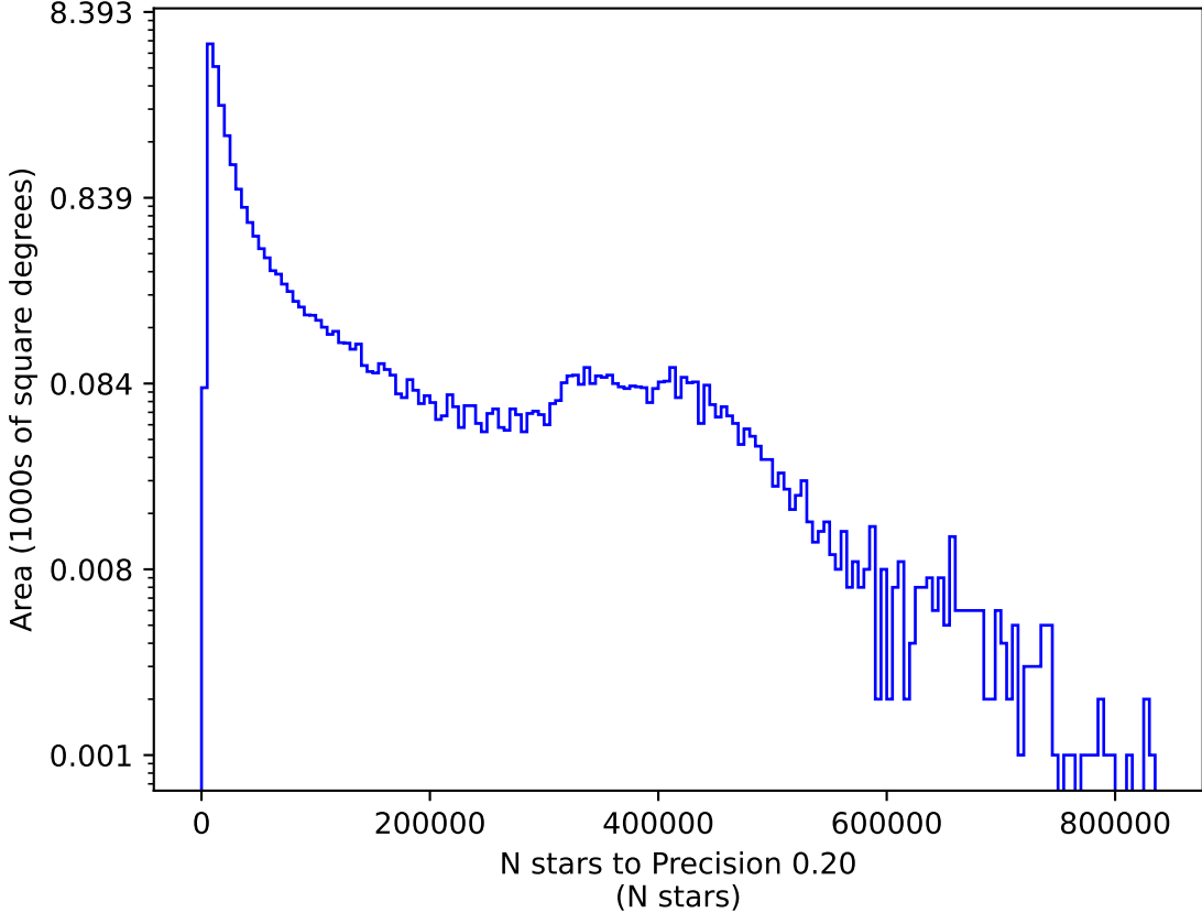
too_elab_heavy_r32_d2_gz_v3.4_10yrs i: N stars to Precision 0.20
