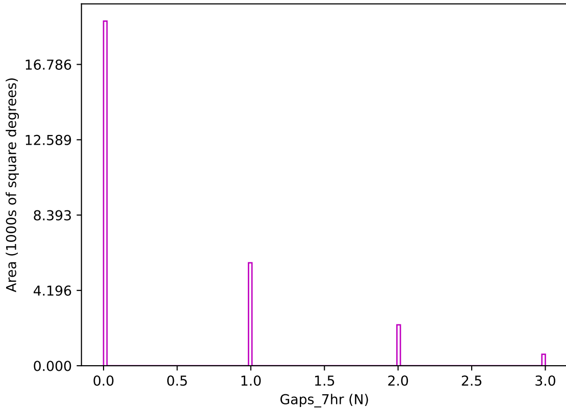
too_elab_heavy_r32_d2_gz_v3.4_10yrs z band: Gaps_7hr
