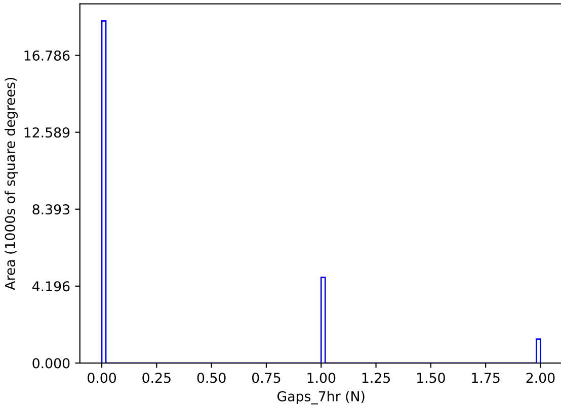
too_elab_heavy_r32_d2_gz_v3.4_10yrs y band: Gaps_7hr
