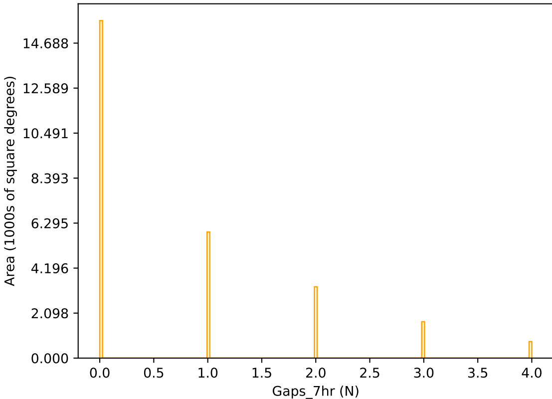
too_elab_heavy_r32_d2_gz_v3.4_10yrs r band: Gaps_7hr
