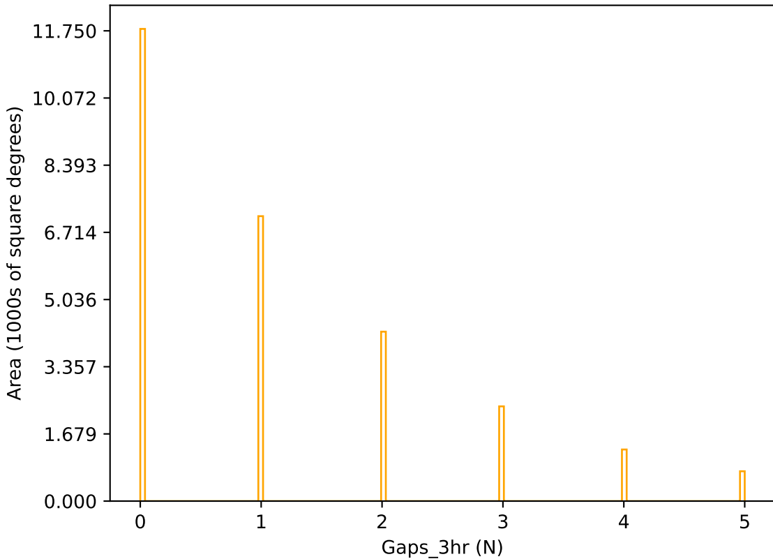
too_elab_heavy_r32_d2_gz_v3.4_10yrs r band: Gaps_3hr
