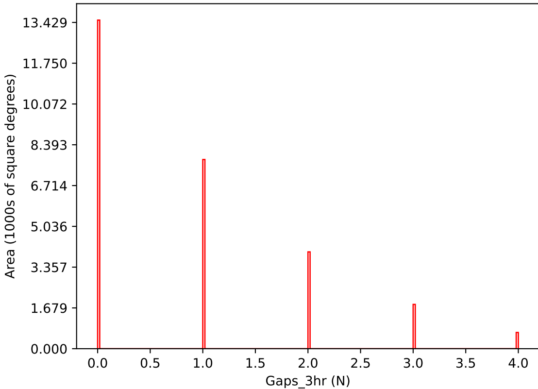
too_elab_heavy_r32_d2_gz_v3.4_10yrs i band: Gaps_3hr
