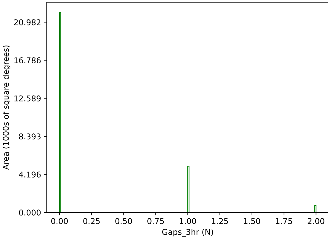
too_elab_heavy_r32_d2_gz_v3.4_10yrs g band: Gaps_3hr
