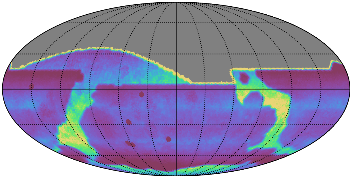
too_elab_heavy_r32_d2_gz_v3.4_10yrs : DCRprecision
