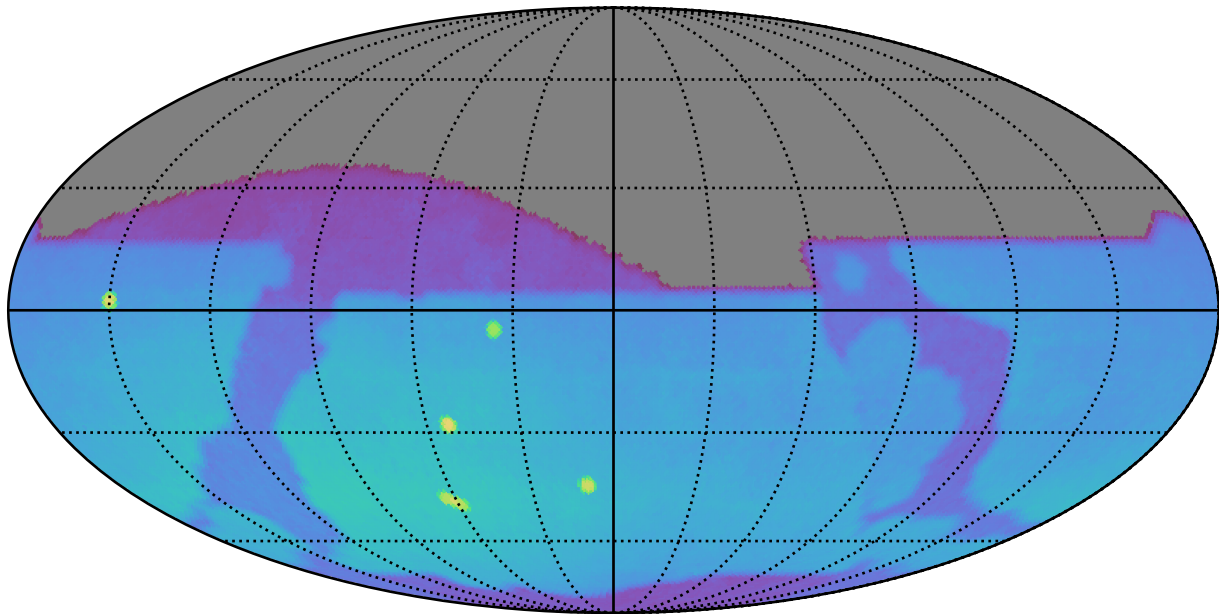
too_elab_heavy_r32_d2_gz_v3.4_10yrs : Brown Dwarf, L4
