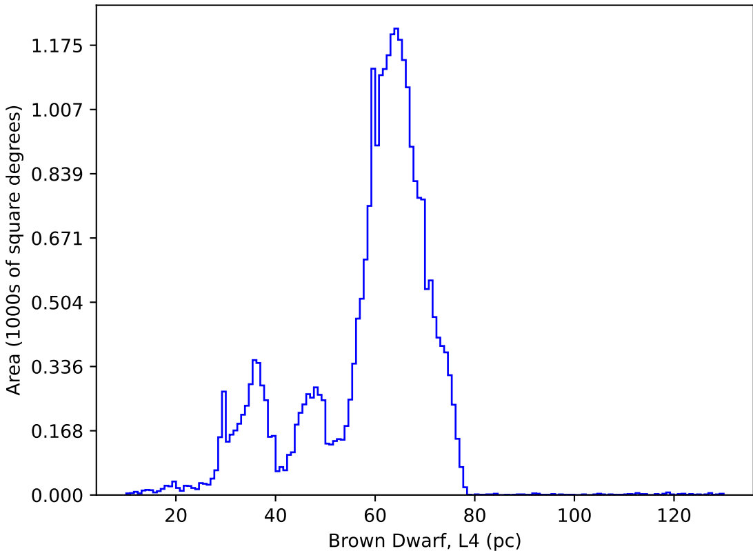
too_elab_heavy_r32_d2_gz_v3.4_10yrs : Brown Dwarf, L4
