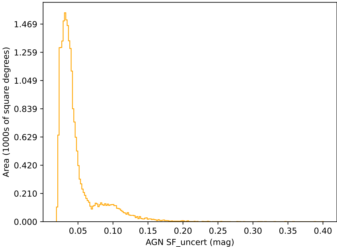
too_elab_heavy_r32_d2_gz_v3.4_10yrs r band: AGN SF_uncert
