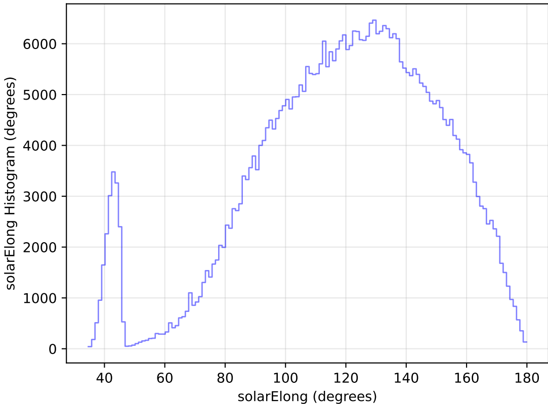
too_elab_heavy_r32_d2_gz_v3.4_10yrs WFD z band: solarElong Histogram
