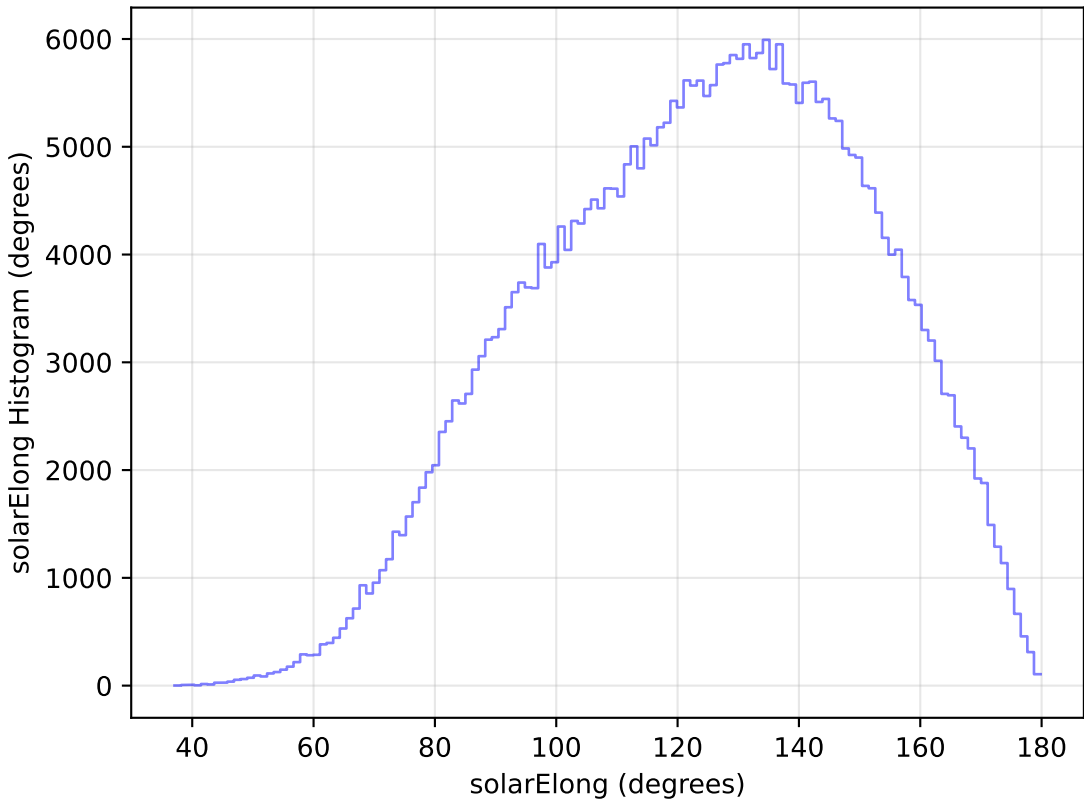
too_elab_heavy_r32_d2_gz_v3.4_10yrs WFD y band: solarElong Histogram
